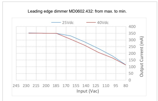
Leading Edge Dimmer MD0602.432: Maximum to Minimum Dimming Curve
