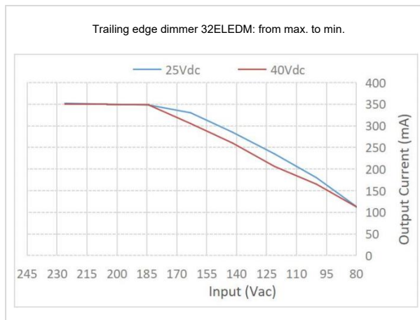
Trailing Edge Dimmer 32ELEDM: Maximum to Minimum Dimming Curve
