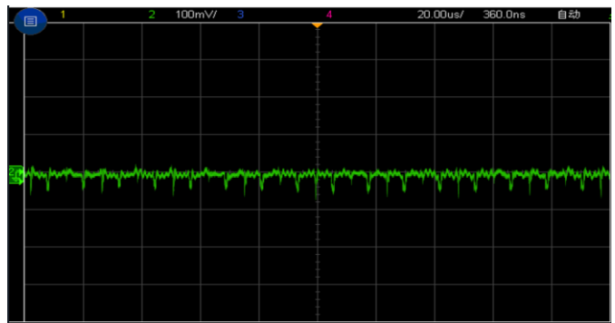
Figure 7, Output ripple & noise (Iout = 10A)
